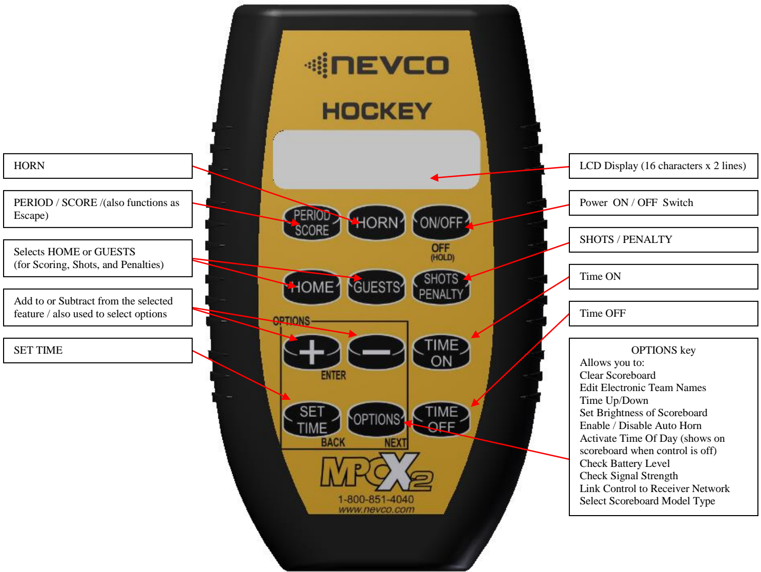
MPCX2 HOCKEY CONTROL (front view)
